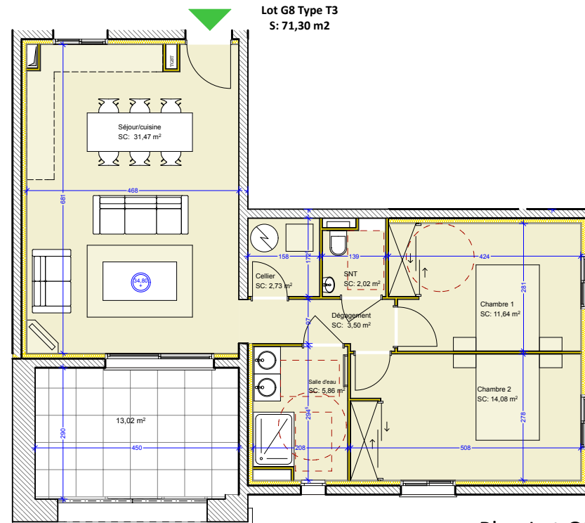
Plan Lot G8
