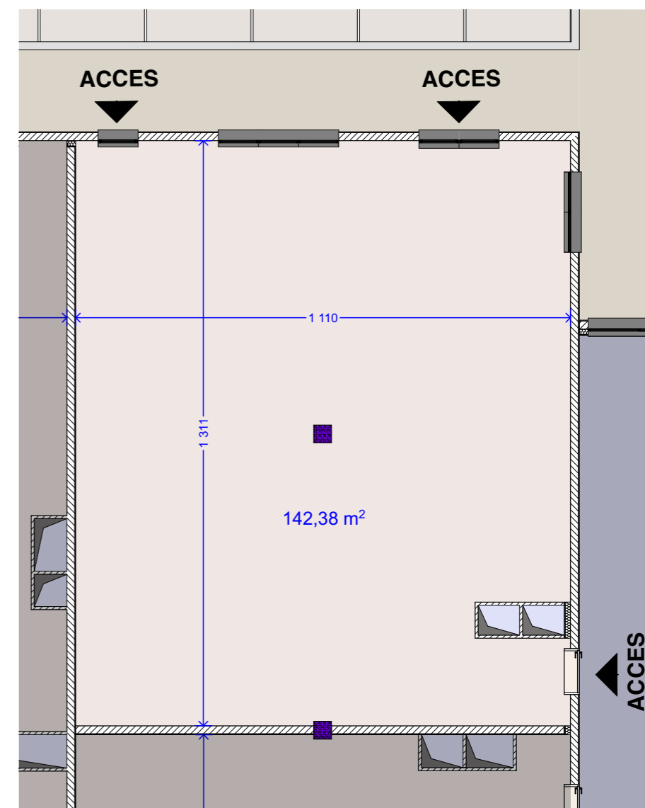
PLAN LOT 002
